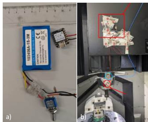
FIGURA 2 a) Device Wiring; b) Device setup.
