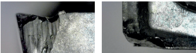
Tool wear after 39 minutes of machining
